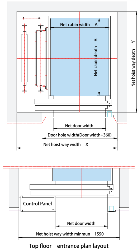
Hoist way plan layout
