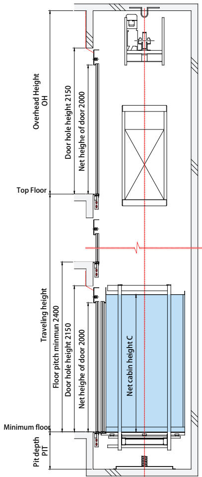
Hoist way vertical section
